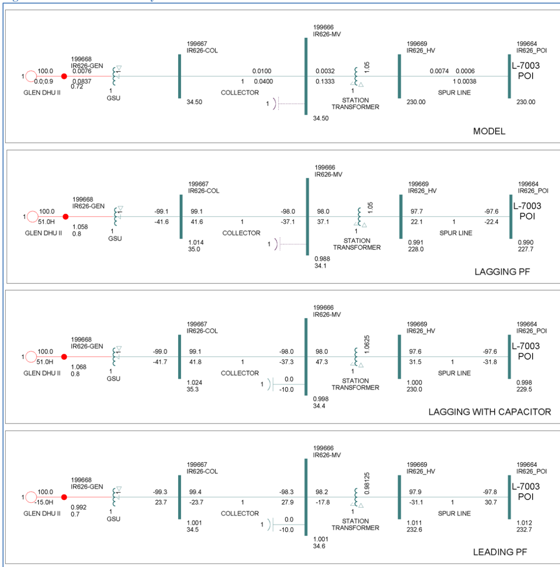
Figure 7: Power Factor Analysis
