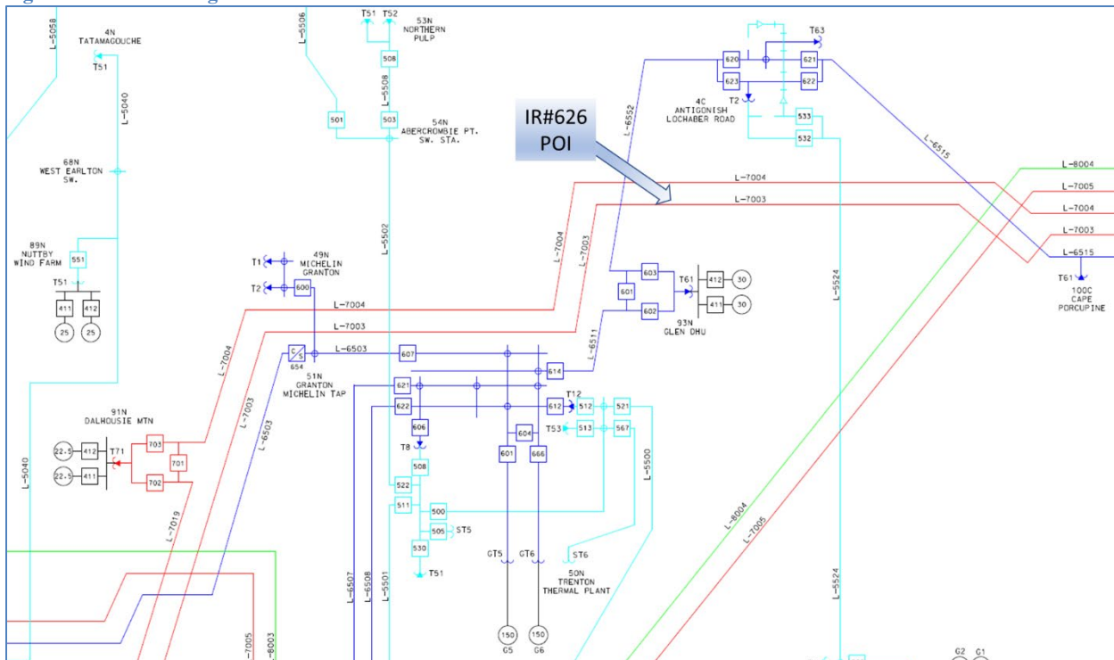
Figure 3 Circuit Configuration near POI
